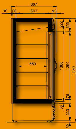
ADR-6 / ADC-6 DIMENSIONS IN mm
