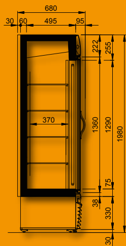
ADR-4 / ADC-4 DIMENSIONS IN mm
